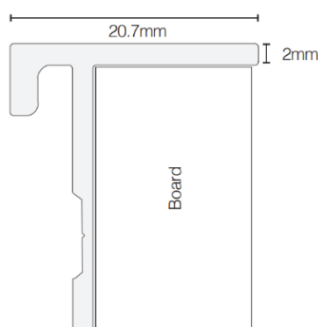
SIDE DETAIL
