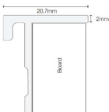
SIDE DETAIL
